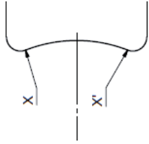
102.6.- Radius for whole upper surface zone BB' to FF'
